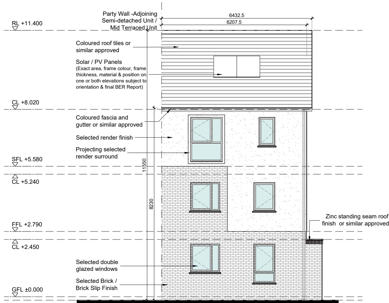
01 Front Elevation
