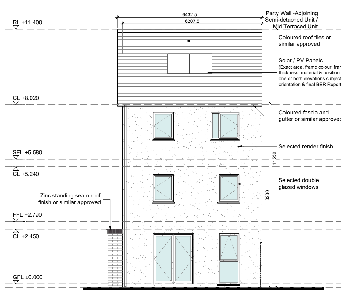
02 Rear Elevation
