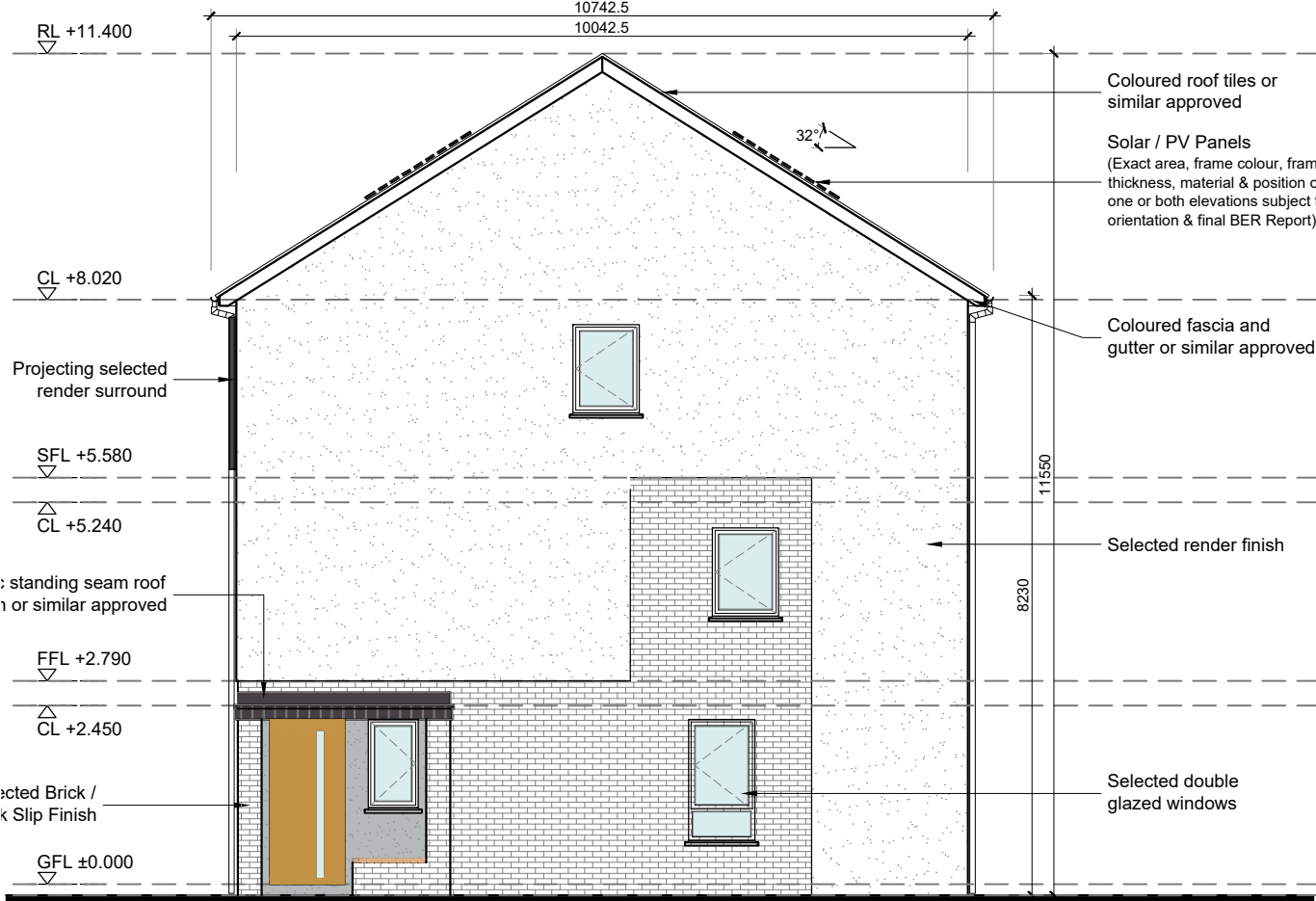
03 Side Elevation
