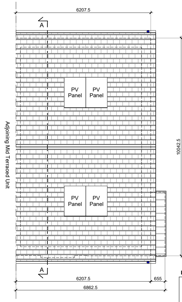
03 Roof Plan 1:100 @ A3
