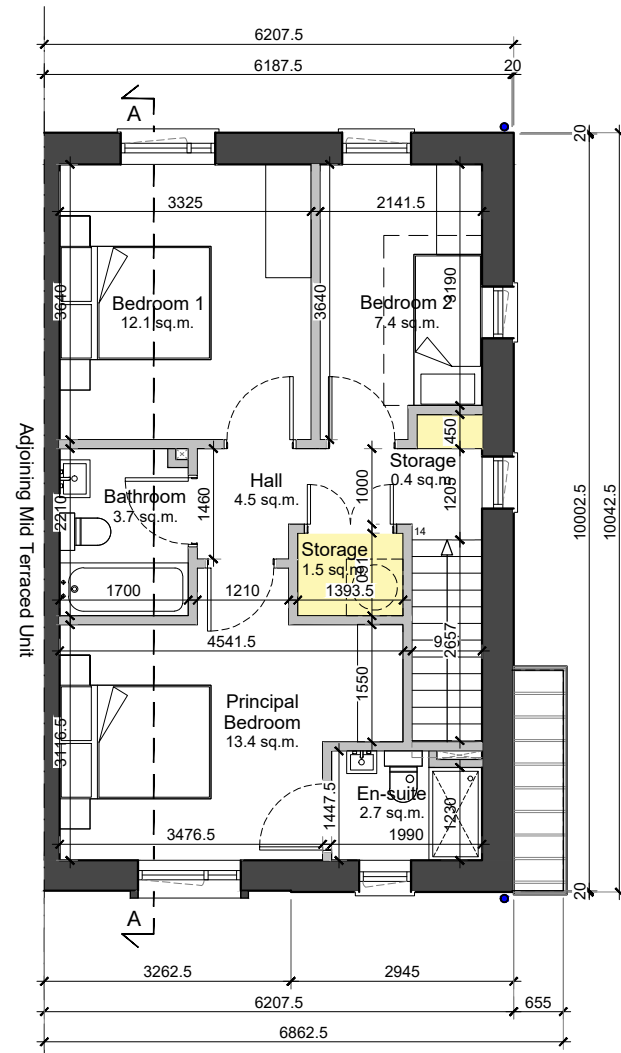
02 First Floor Plan 1:100 @ A3
