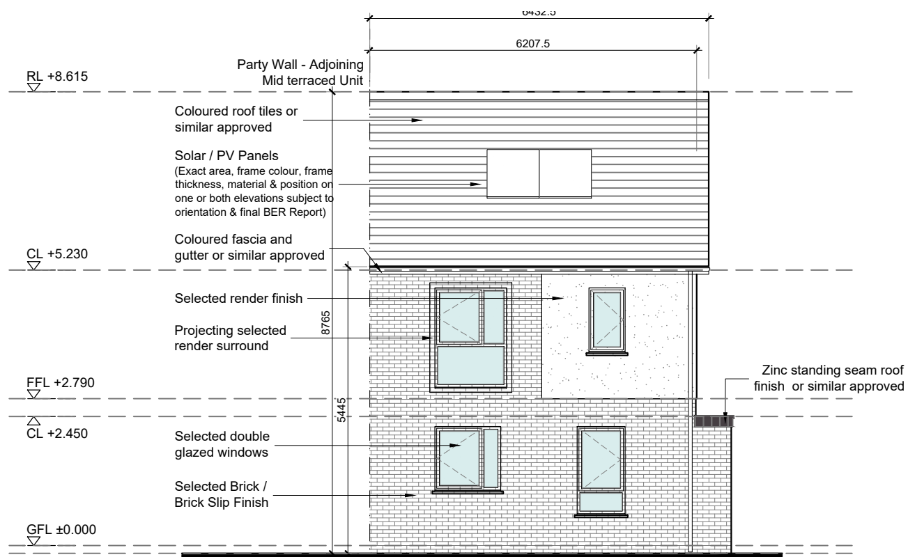
01 Front Elevation 1:100 @ A3
