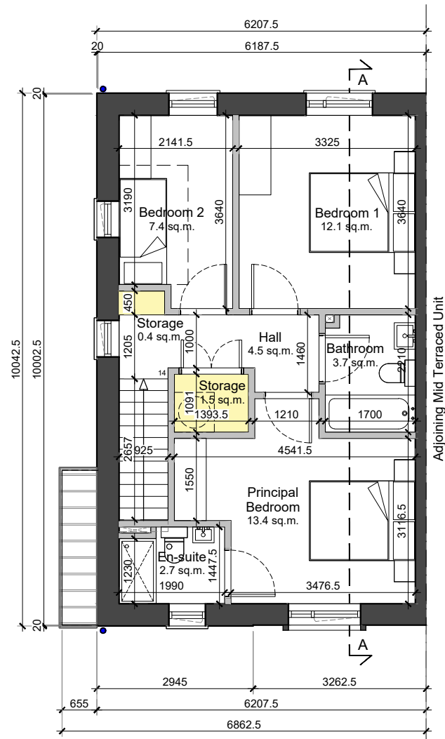
02 First Floor Plan 1:100 @ A3
