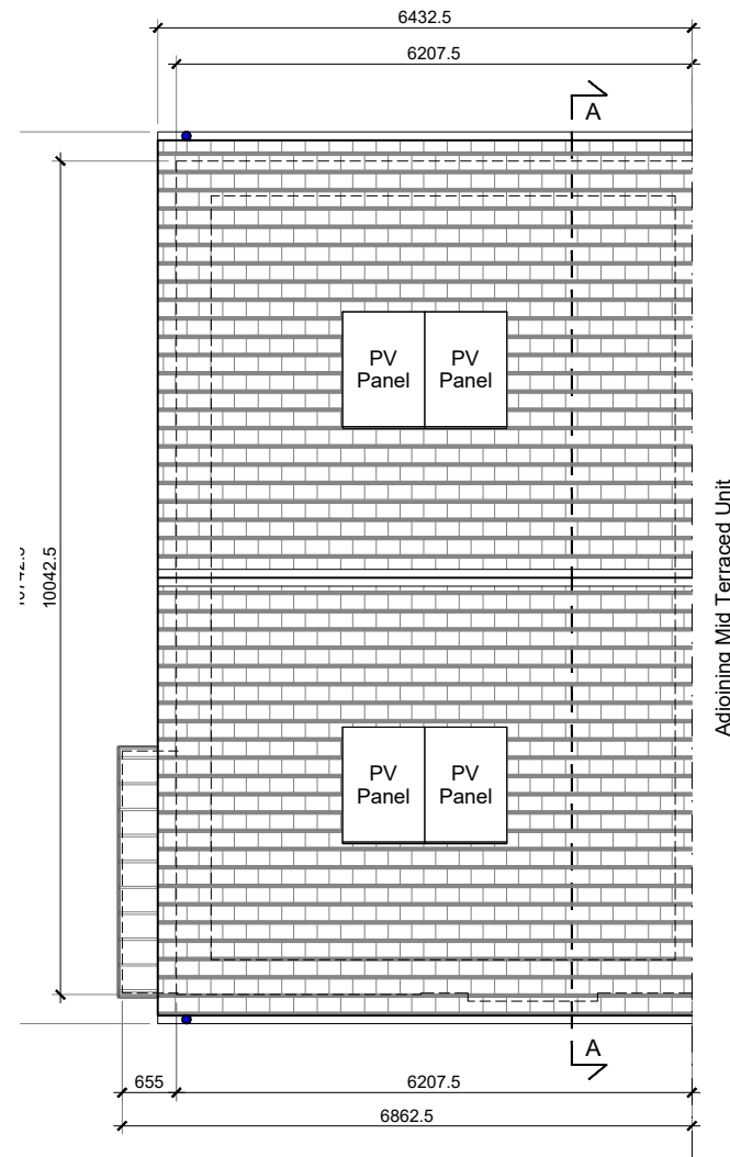
03 Roof Plan 1:100 @ A3
