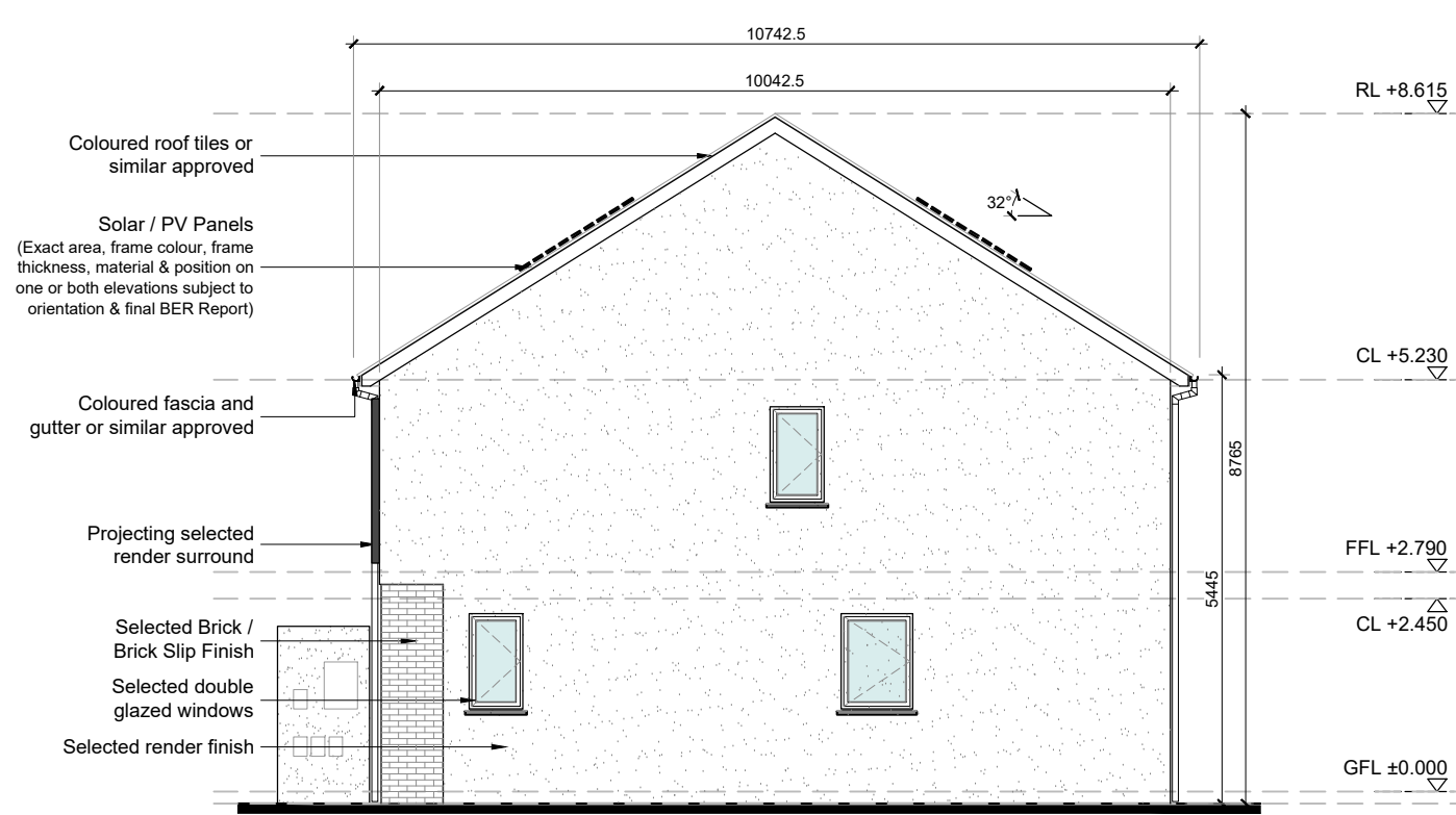
03 Side Elevation 1:100 @ A3
