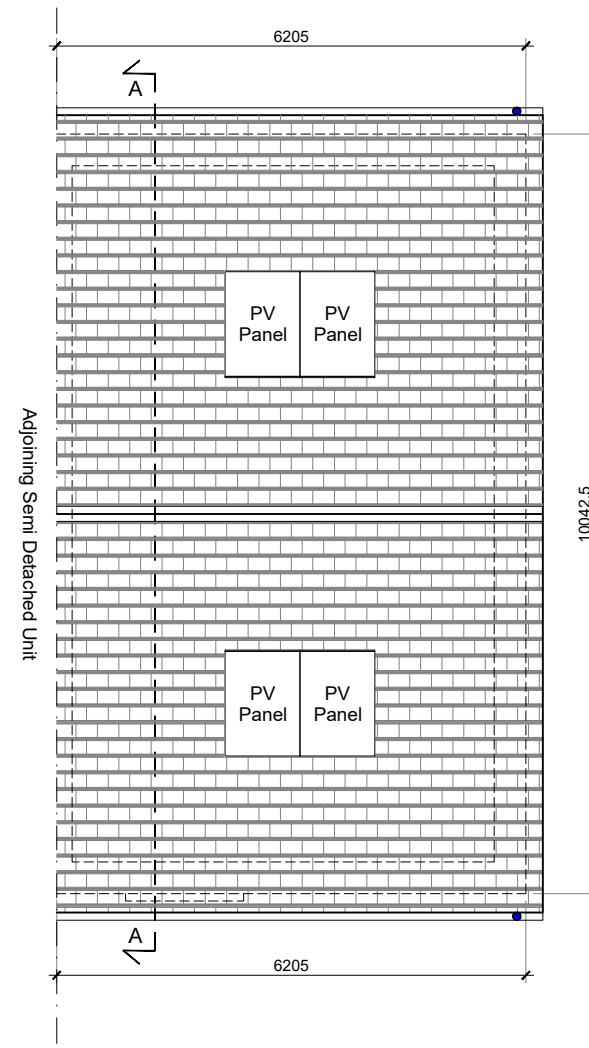
04 Roof Plan 1:100 @ A3
